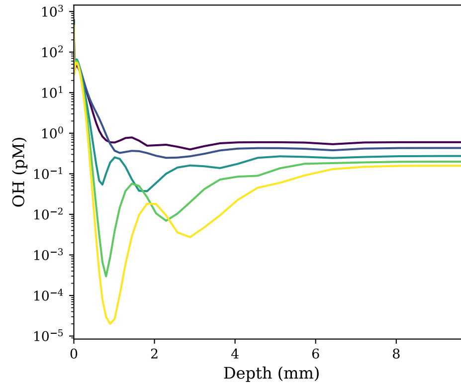
(e) OH
