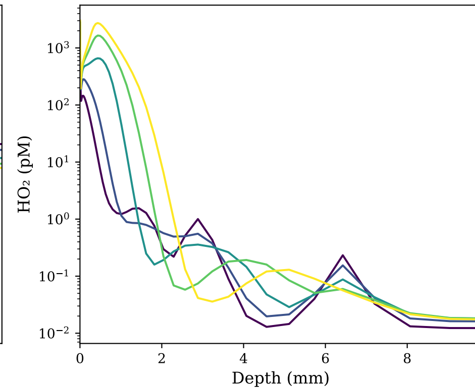
(f) \text{HO}_2
